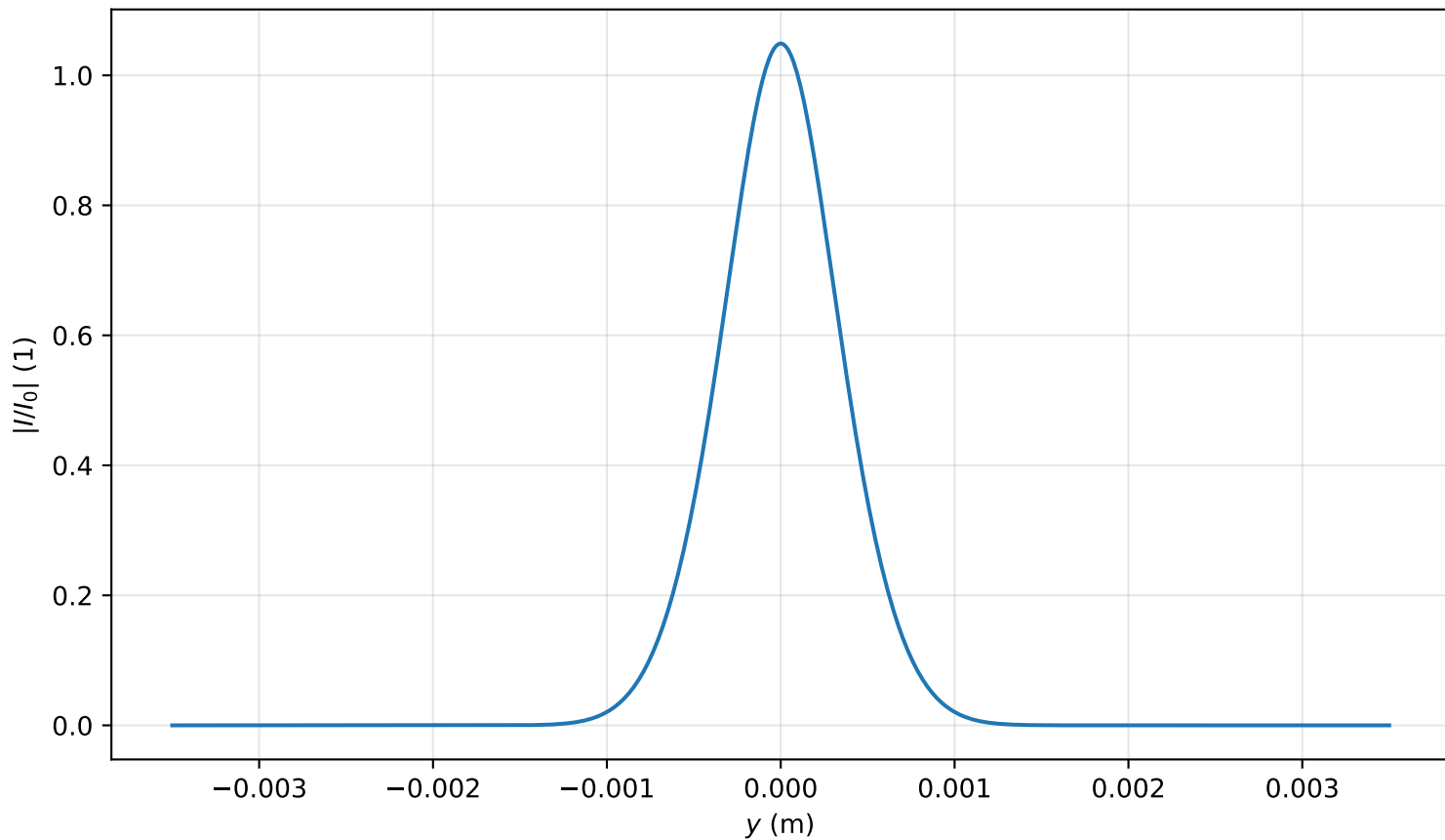
Intensity profile I(x=0, y, z=0.557)/I_0 , P_{in}=0.5P_{cr} , artificial time
